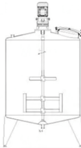
Frame Mixing
